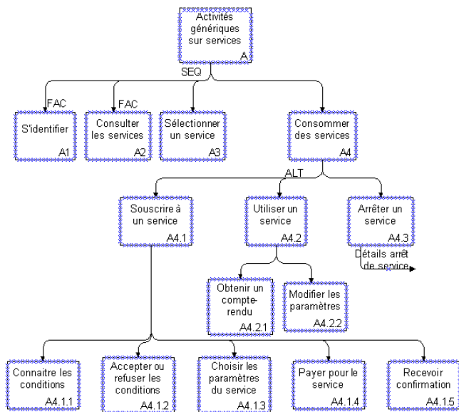
Fig 1: Schematic representation of the hierarchical task model for generic tasks
